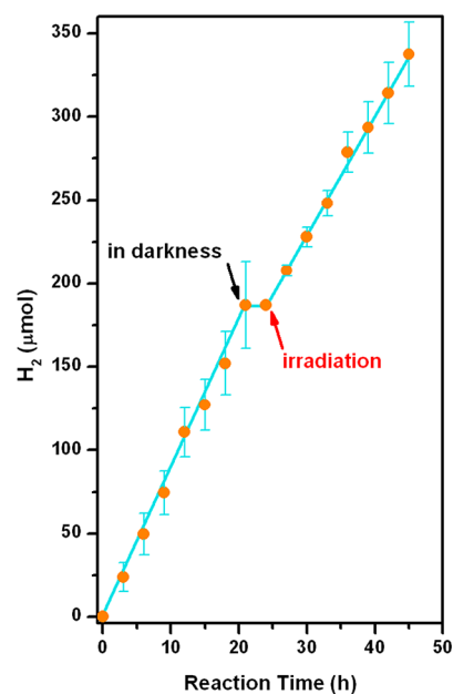
Figure 8. Photosynthetic \text{H}_2 production from \text{Ni}_h -CdTe hollow nanospheres in 10 mL of a 5.68 \times 10^{-2} M (100 mg/10 mL) \text{H}_2\text{A} aqueous solution (pH = 4.65) under visible light irradiation ( \lambda > 400 nm). Error bars represent the mean \pm s.d. of three independent experiments.
