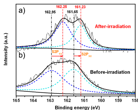
Figure 3. S 2p XPS spectra recorded from (a) Ni h -CdTe hollow nanospheres and from (b) MPA-CdTe QDs; the vertical lines are guides for the positions of S 2p 1/2 and S 2p 3/2 from MPA-Cd and CdS, respectively.
