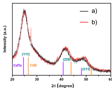
Figure 2. XRD patterns of (a) MPA-CdTe QDs and (b) Ni h -CdTe hollow nanospheres.
